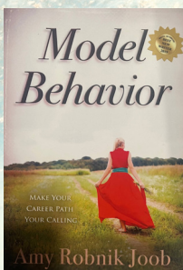
Model Behavior
